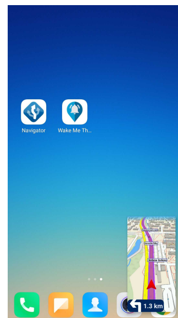
Picture-in-picture Modus
